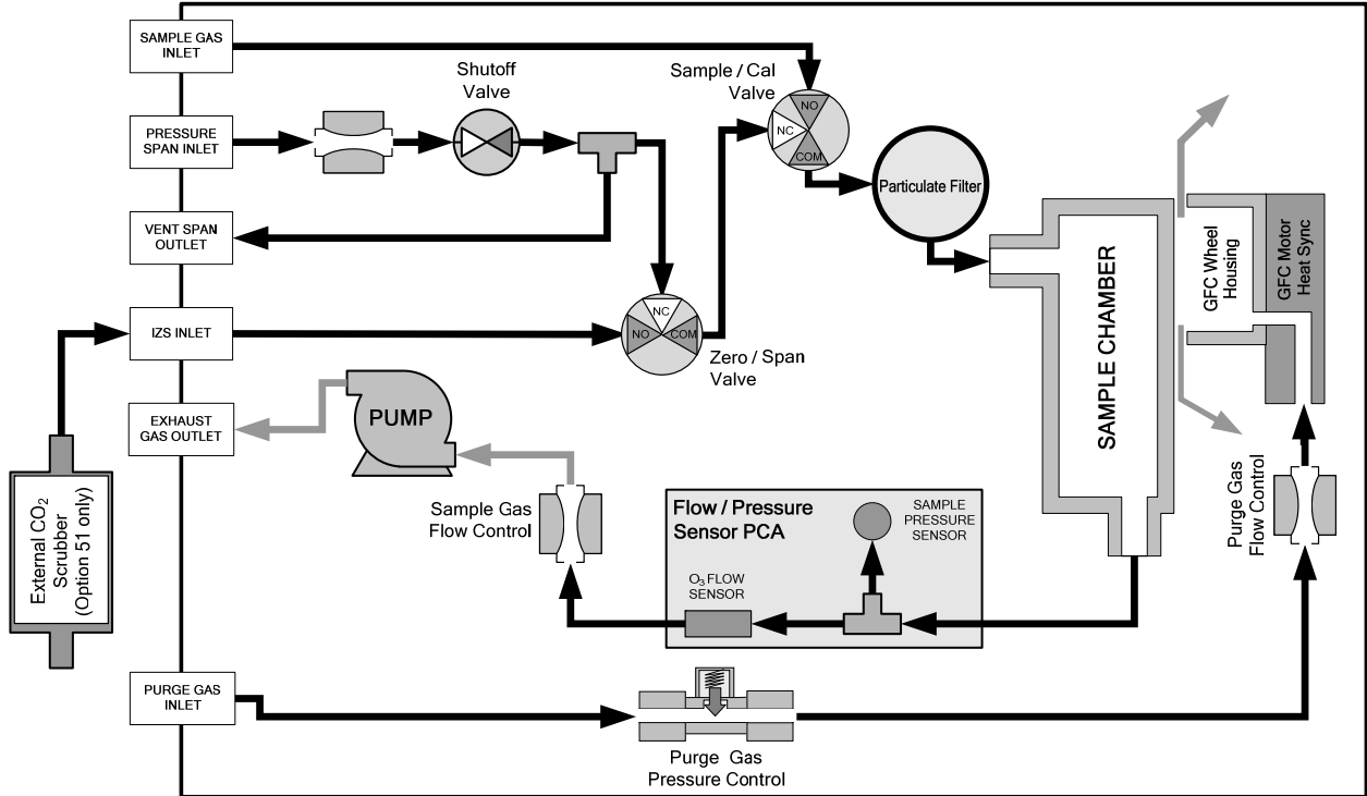
Figure 8-7: Internal Pneumatic Flow – Ambient Zero/Pressurized Span Valves
